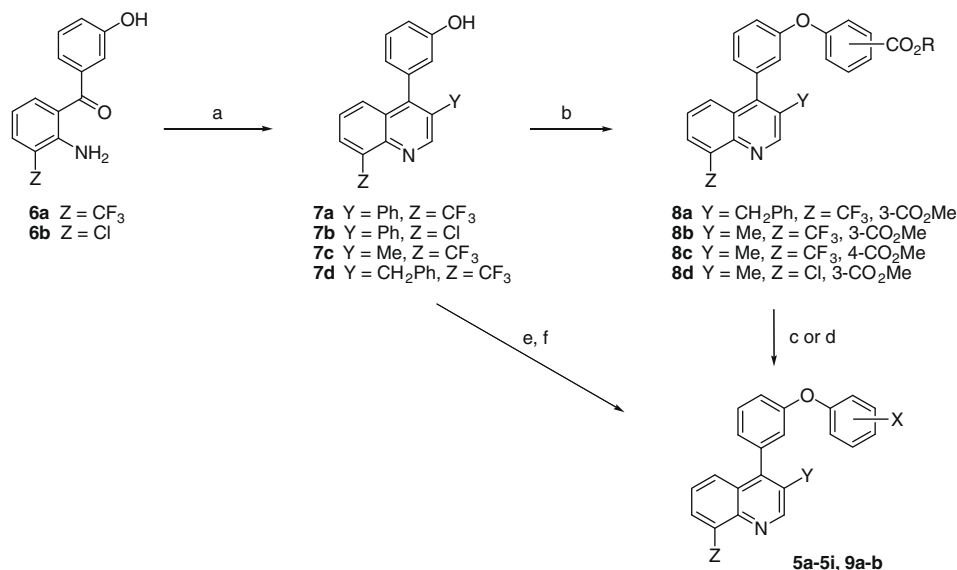
Scheme 1. Reagents and conditions: (a) PhCH 2 CHO, PhSO 3 H, toluene (Y = Ph) or MeCH 2 CHO, cat. H 2 SO 4 , AcOH (Y = Me), heat, 3–24 h (63–79%); (b) BrPhCO 2 R, CuI, Me 2 NCH 2 CO 2 H·HCl, Cs 2 CO 3 , dioxane, 105 °C (64–78%); (c) R 1 MgX, THF (82–92%); (d) LiBH 4 , THF (72–97%); (e) ArB(OH) 2 , Cu(OAc) 2 , Et 3 N, microwave or heat (36–76%); (f) pyridine hydrochloride, 180–190 °C, 3 h (90%).
